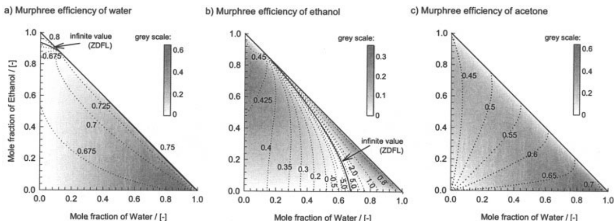
Figure 3. Component Murphree efficiencies of the ethanol–water–acetone system.
